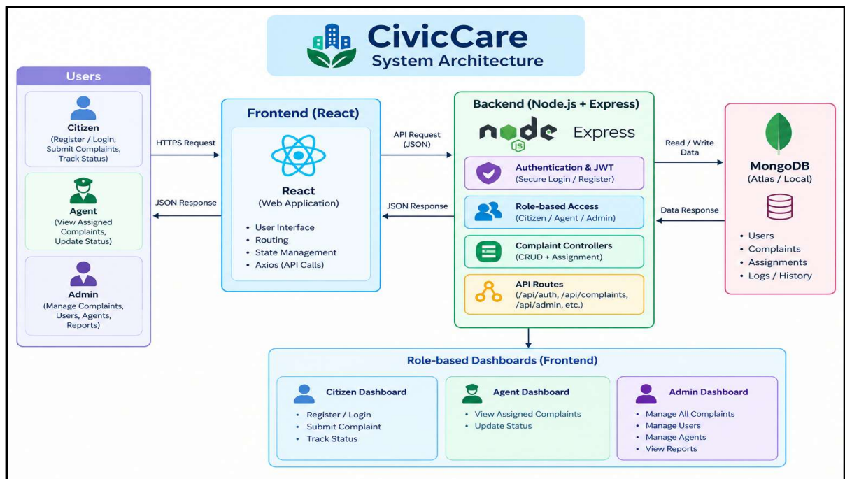
Figure 1: Architecture and data flow of the CivicCare online complaint management system
